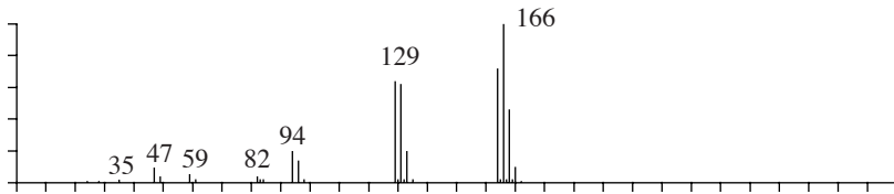
Dibutyl phthalate [25] (frequent impurity due to its use as polymer plasticizer)
