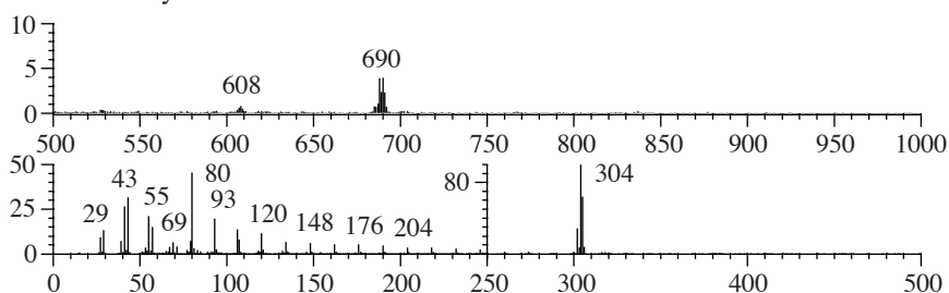
Hexadecylpyridinium bromide ( M_r 384.4; for [hexadecylpyridinium] ^+ m/z 304.3) in 2-nitrobenzyl alcohol
